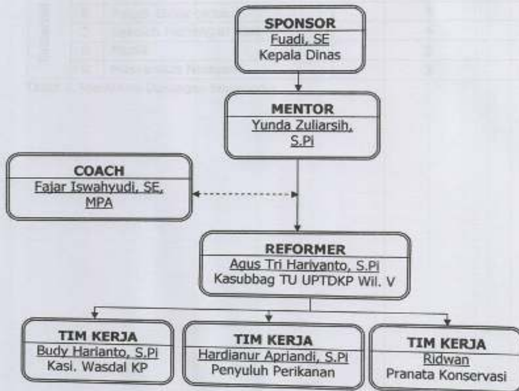
Gambar 3. Skema Stakeholder
